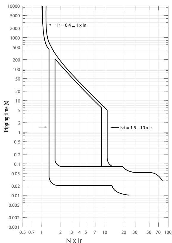
NBS-E (100 - 630A) I/t characteristic
