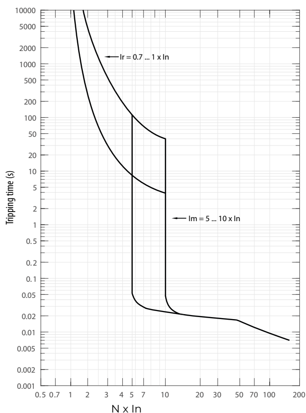
NBS-TMD 630/3 (500, 600A) I/t characteristic
