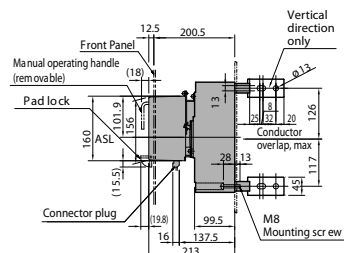
Rear connected with Motor Operator
