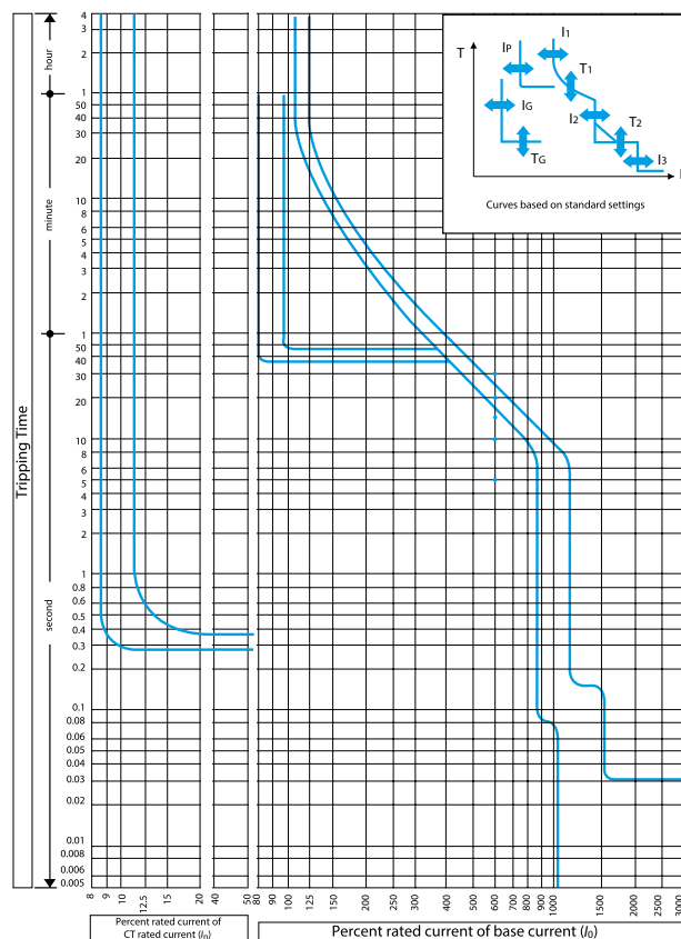
Time/current characteristic curves EB2 630-VE, EB2 800-VE
