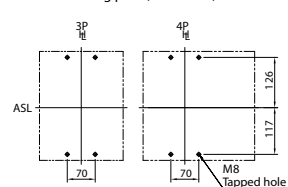
Drilling plan (front view)
